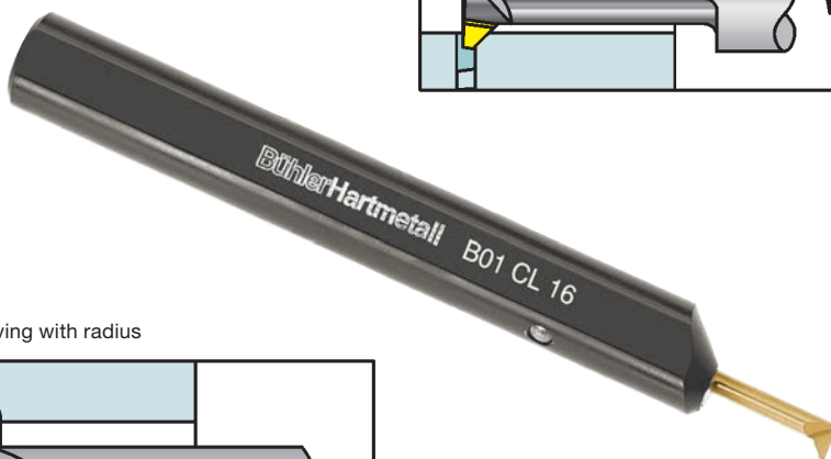
Reverse turning
