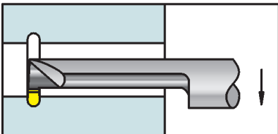
Grooving with radius
