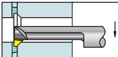
Pre-grooving and chamfering
