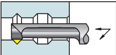
Recessing and chamfering
