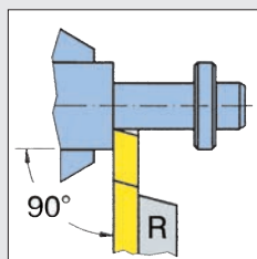
Turning Cut-off operation
