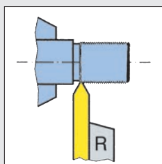
Partial thread
